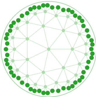
(a) \{3, 7\}, L = 56
