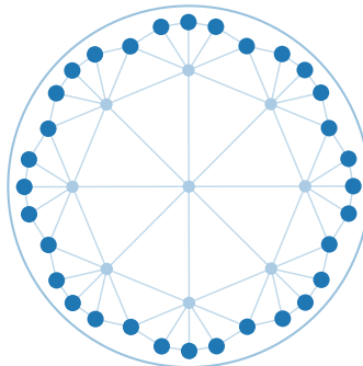
(b) \{3, 8\}, L = 32
