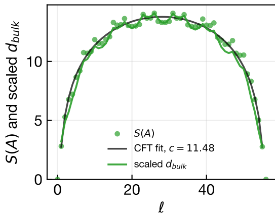
(c) \mu = 0.1
