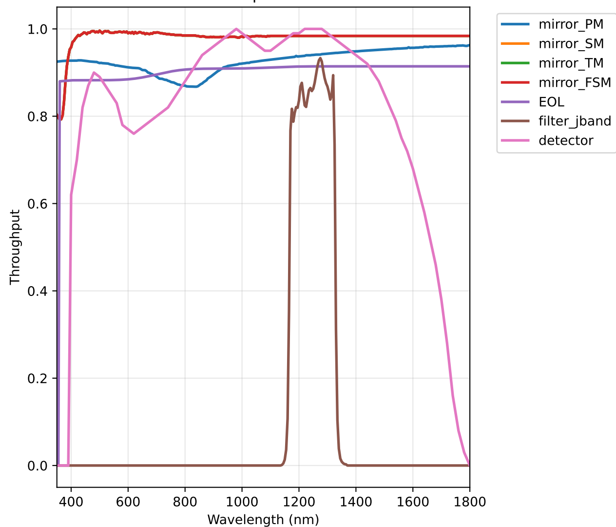
Subsystem Throughputs
