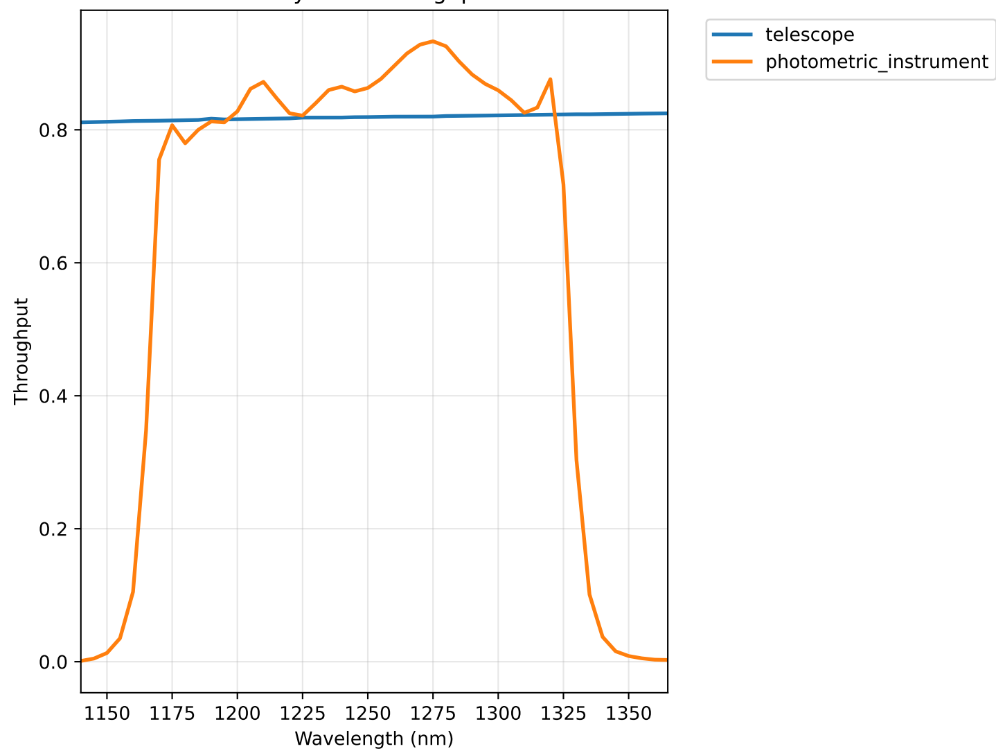
Subsystem Throughputs
