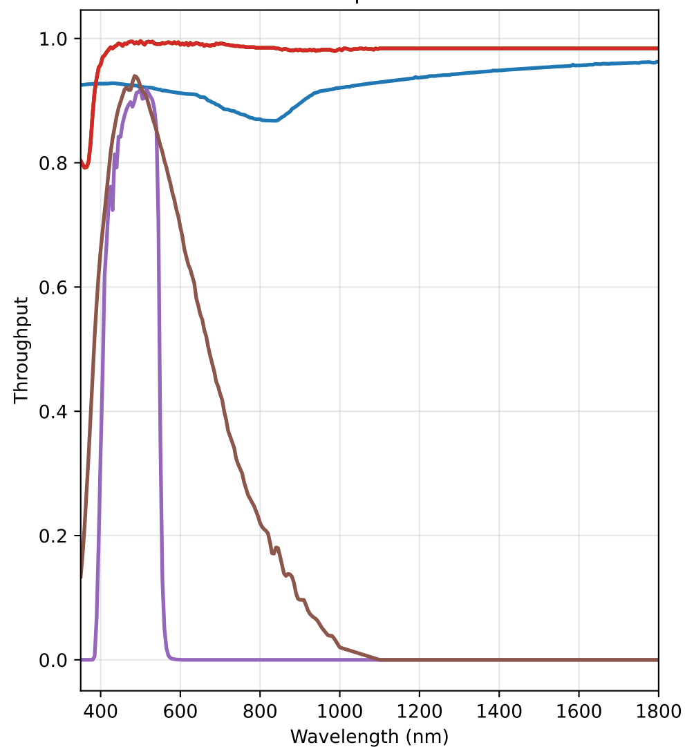
Subsystem Throughputs
