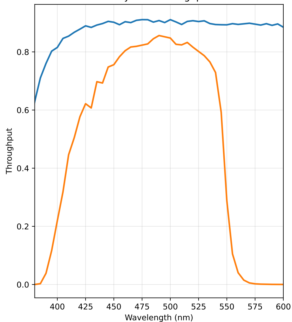
Subsystem Throughputs
