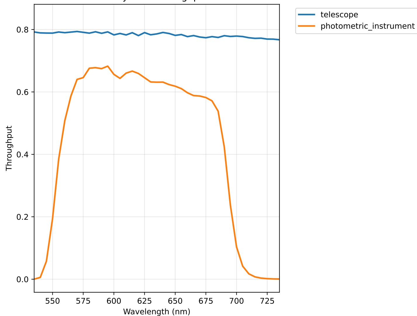
Subsystem Throughputs
