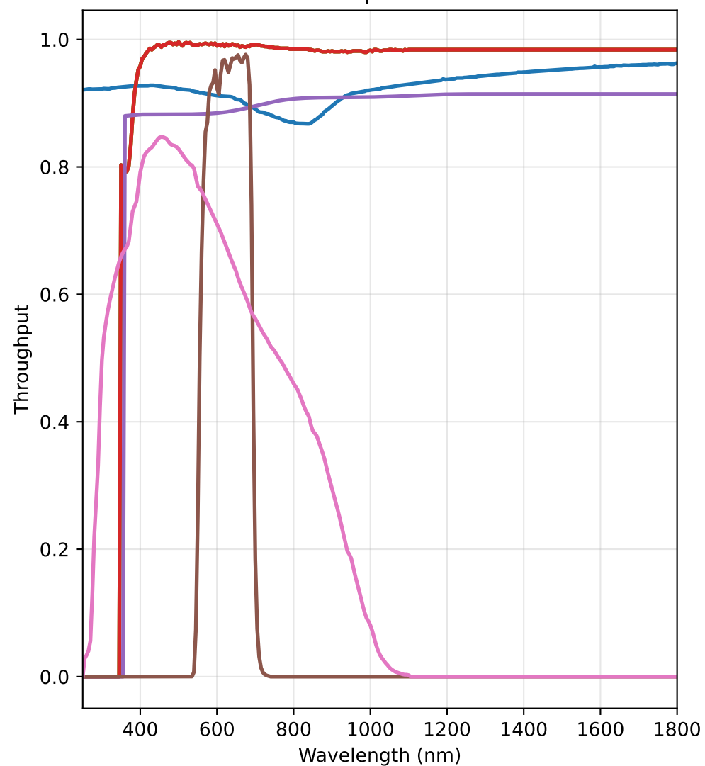
Subsystem Throughputs
