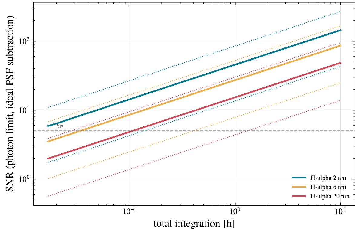
PDS 70 b: 160 mas, F = 8.1\text{e-}16 (dotted: 2.3\text{e-}16 , 1.6\text{e-}15 )
