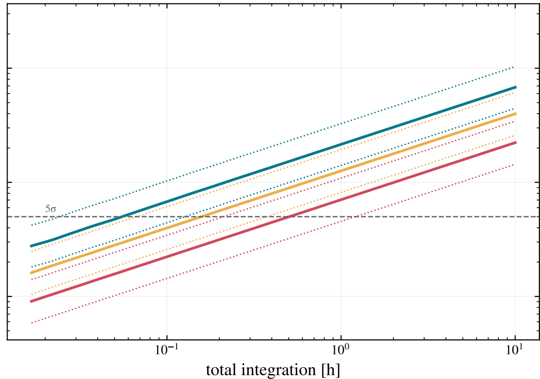
PDS 70 c: 210 mas, F = 3.1\text{e-}16 (dotted: 2.0\text{e-}16 , 4.8\text{e-}16 )
