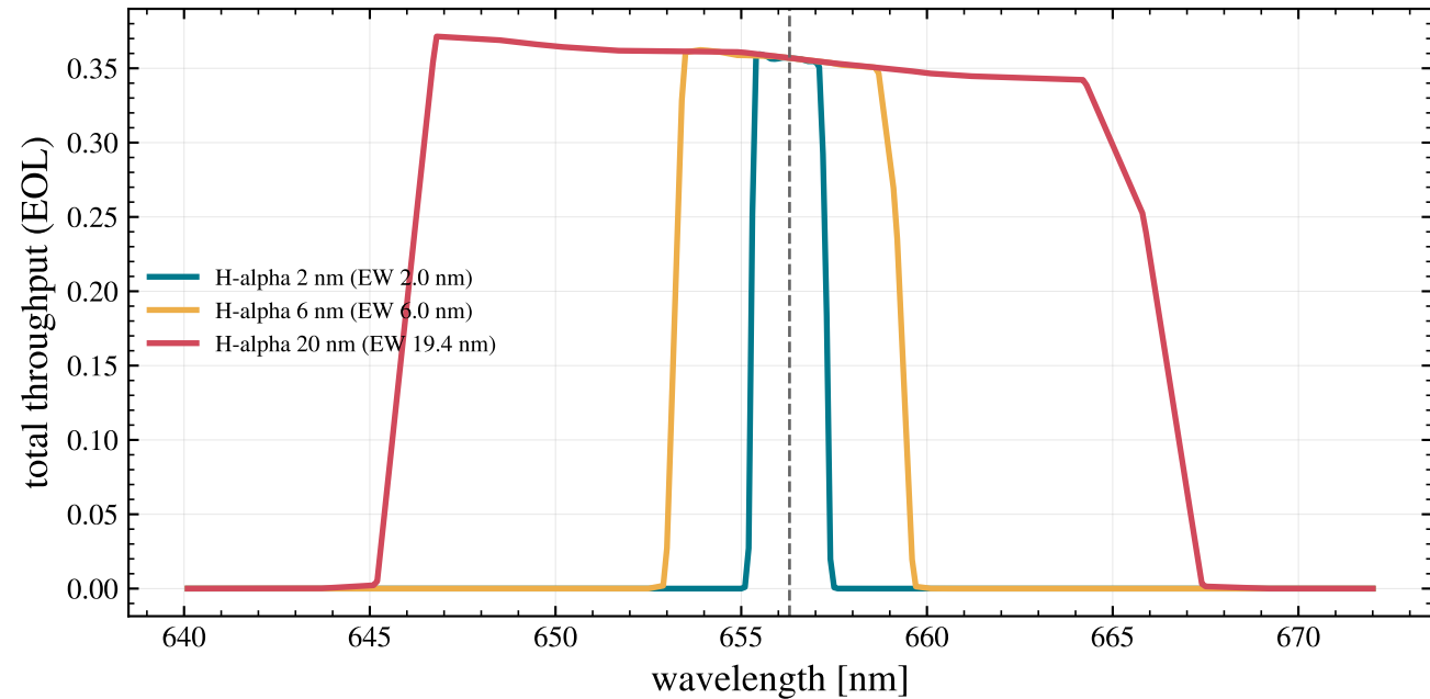
WCC H-alpha filters as in the ETC (IMX455 channel)
