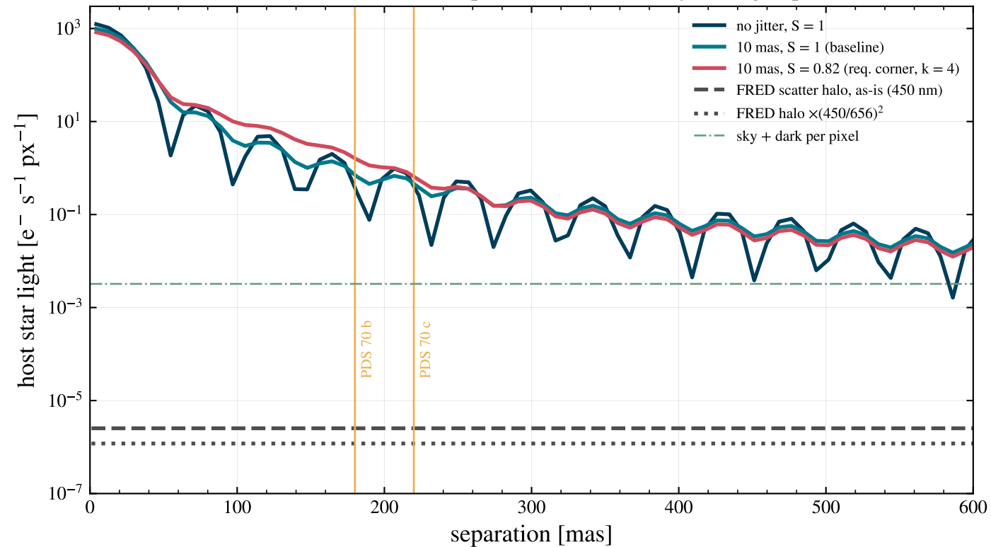
K7V G = 11.7 host in H-alpha 2 nm: azimuthally averaged profile
