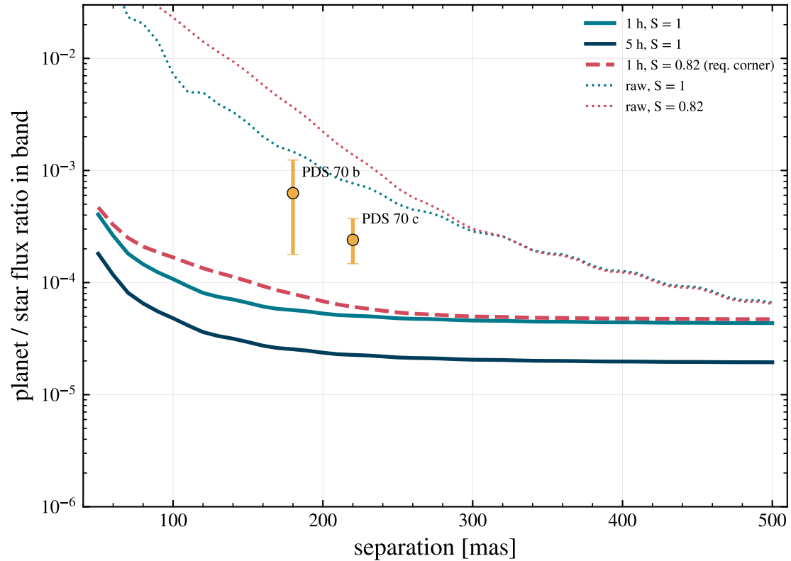
H-alpha 2 nm: time and Strehl; bars = literature flux range
