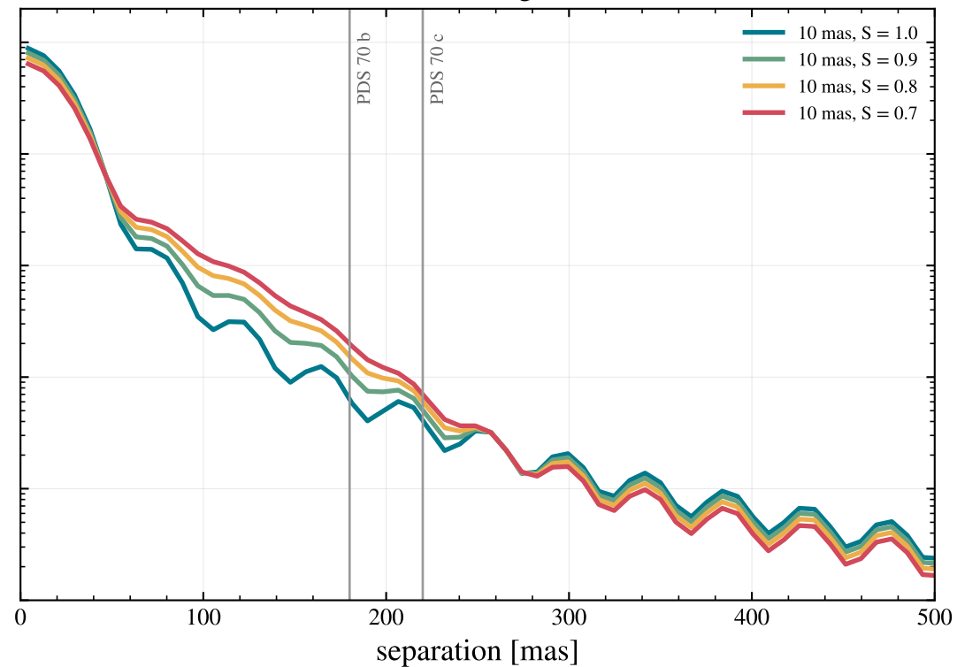
Strehl halo ( k = 4 ) adds light at 100-300 mas
