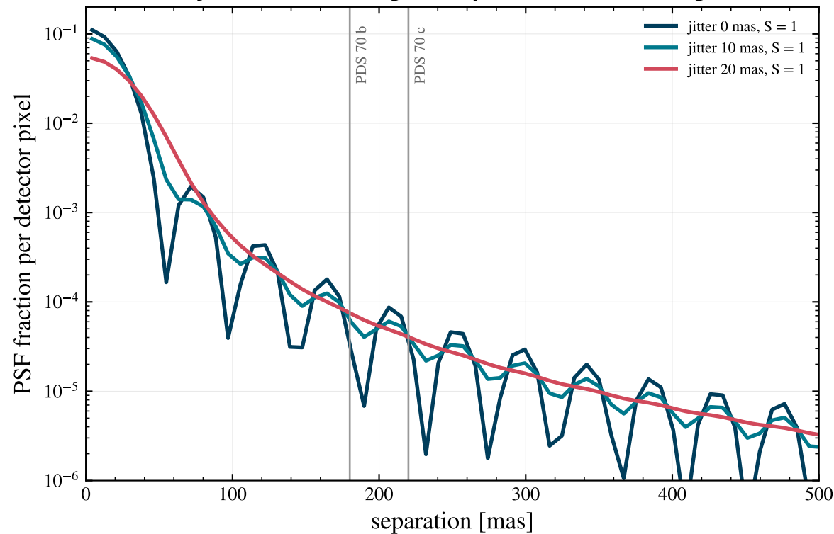
jitter smears the rings, barely moves the mean wing
