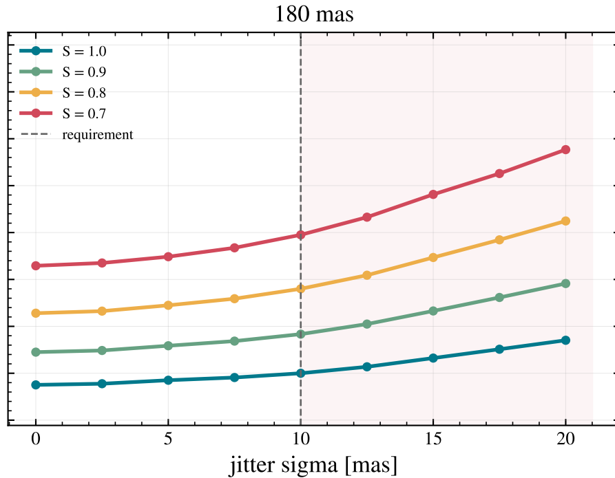
static PSF effect on the photon-noise limit, 2 nm filter, 1 h
