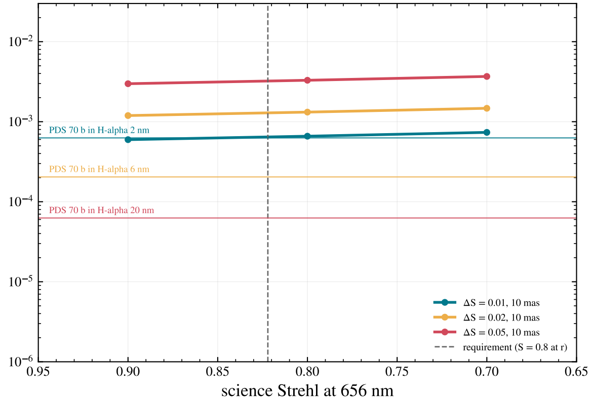
Strehl drift between science and reference, 180 mas ( k = 4 )
