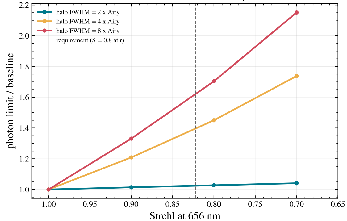
static effect at 180 mas, 10 mas jitter
