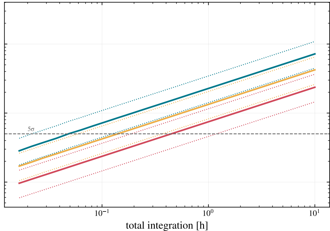
PDS 70 c: 220 mas, F = 3.1\text{e-}16 (dotted: 1.9\text{e-}16 , 4.8\text{e-}16 )
