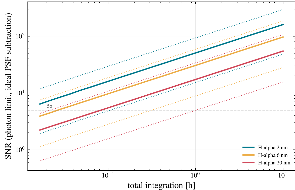
PDS 70 b: 180 mas, F = 8.1\text{e-}16 (dotted: 2.3\text{e-}16 , 1.6\text{e-}15 )
