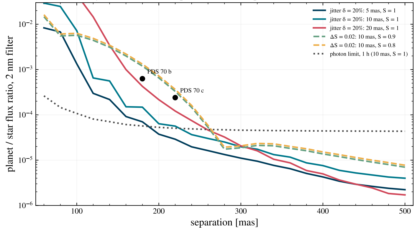
systematic floor vs separation (PDS 70 planets in the 2 nm band)
