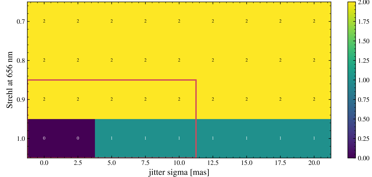
limiting term: 0 photon, 1 jitter mismatch (20%), 2 Strehl drift (0.02)
