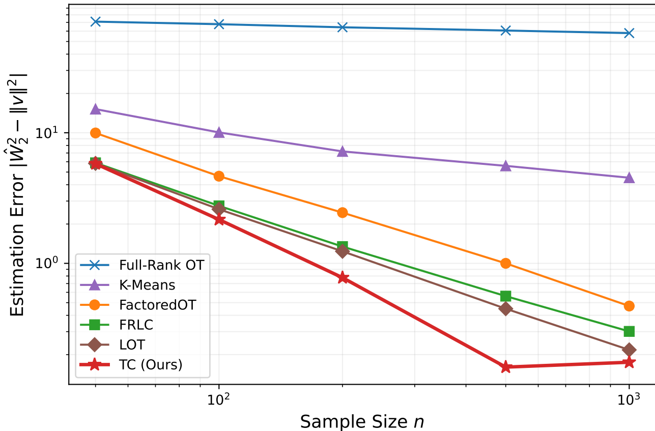
Sample Complexity on Translated GMM ( D=50, K=5, \sigma=1.0 )
