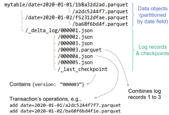
Figure 2.2: The architecture of a Delta Lake table, as presented in [8].
