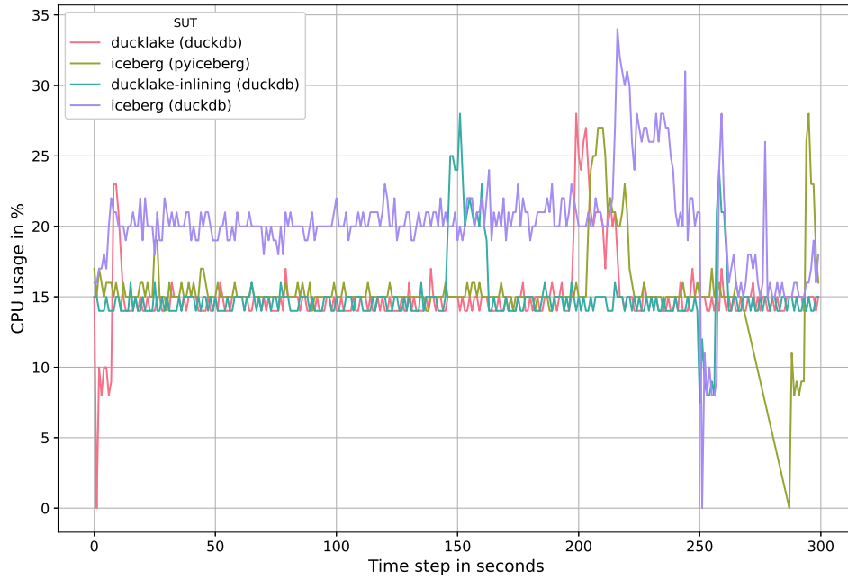
Figure 5.6: CPU usage percentage measured at every second throughout the first hot run of writing individual events to each SUT.
