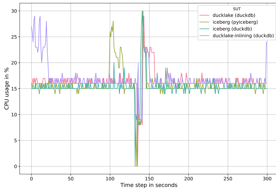
Figure 5.12: CPU usage percentage measured at every second throughout the first hot run of writing batched events to each SUT.
