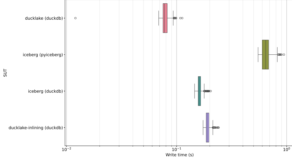
Figure 5.9: Box plots of the time spent writing each batch of 1,000 events to the lakehouse tables during the first hot run, in seconds.
