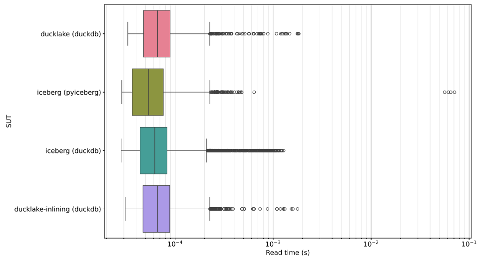
Figure 5.11: Box plots of the time spent reading individual events from Kafka during the first hot run of each SUT, in seconds.
