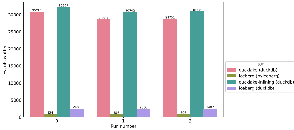
Figure 5.1: Throughput of each SUT in a time span of 5 minutes when writing events one by one. The run numbers correspond to the repetitions of each experiment, where run 0 is considered cold and runs 1 and 2 are considered hot.
