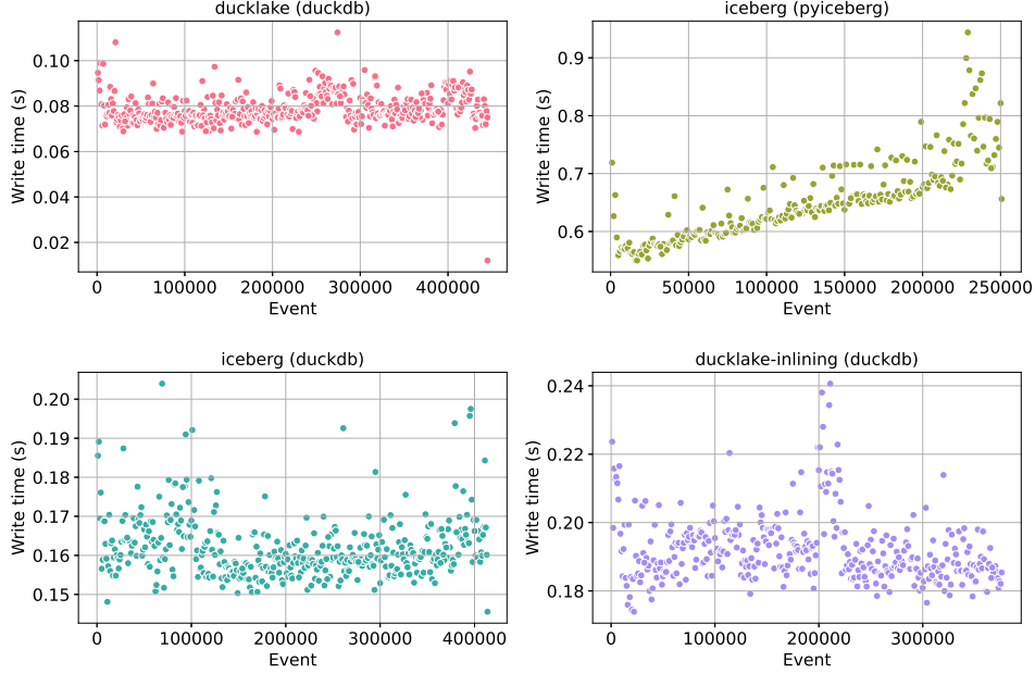
Figure 5.10: Scatter plots of the time spent writing each batch of 1,000 events to each SUT during the first hot run, in seconds.
