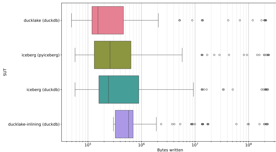
Figure 5.8: Box plots of bytes written to disk at every second when inserting batches of 1,000 events to each SUT (hot run). The measurements were taken at intervals of 1 second.
