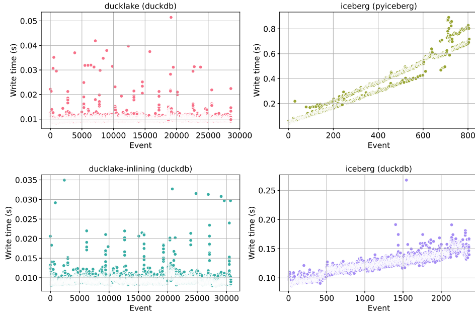
Figure 5.4: Scatter plots of time spent writing individual event to each SUT during the first hot run, in seconds.
