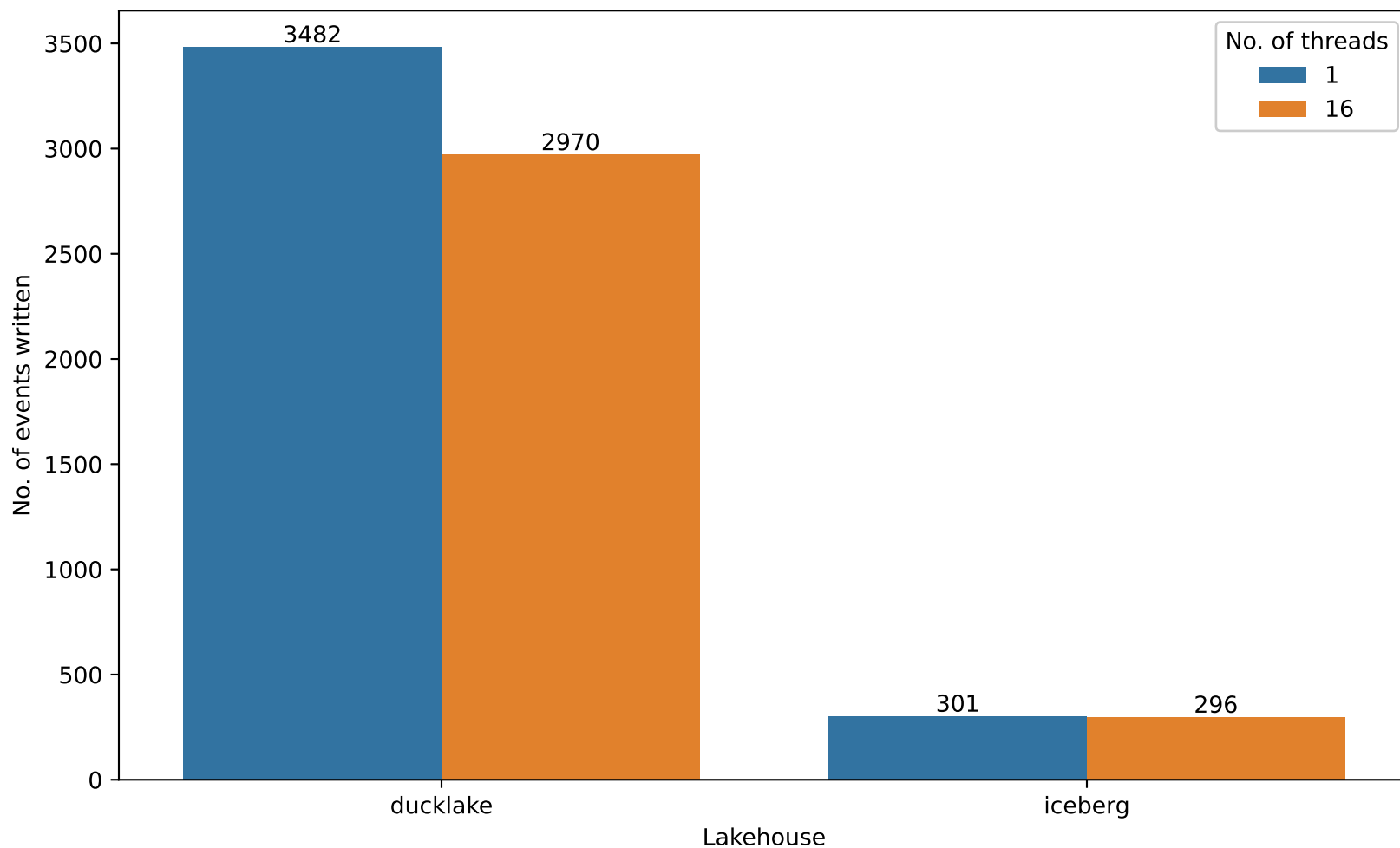
Number of Kafka events written to each lakehouse after 1 minute, using 1 thread vs. 16 threads
