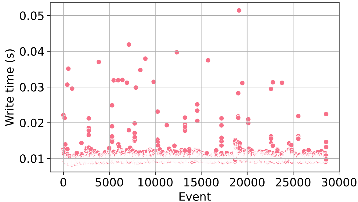
ducklake (duckdb)
