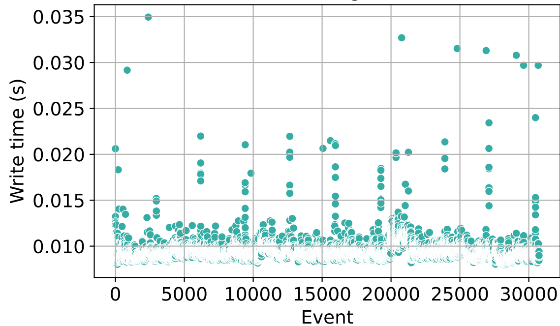
ducklake-inlining (duckdb)
