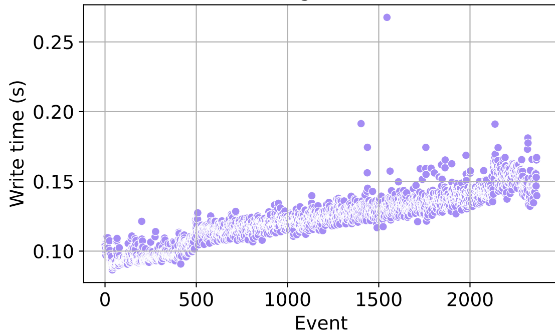
iceberg (duckdb)
