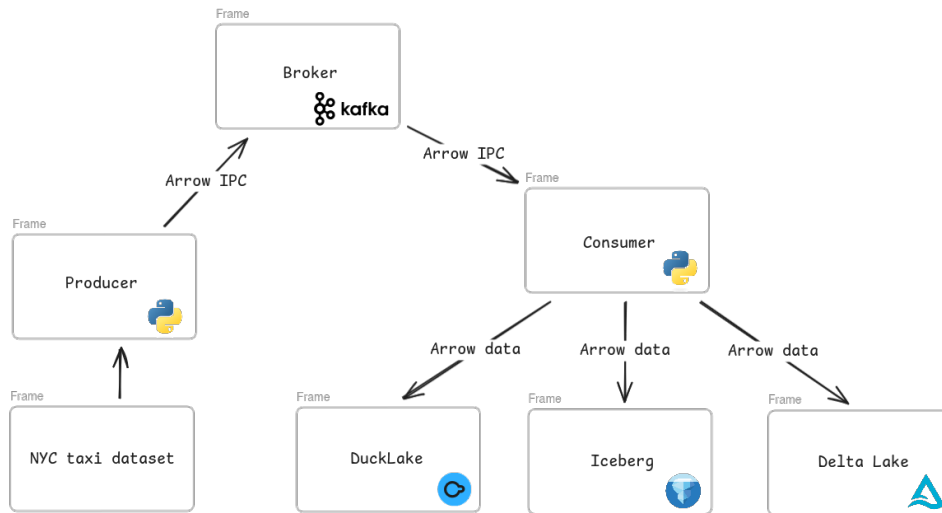
Figure 4.1: Overview of the components in our benchmarking tool.
