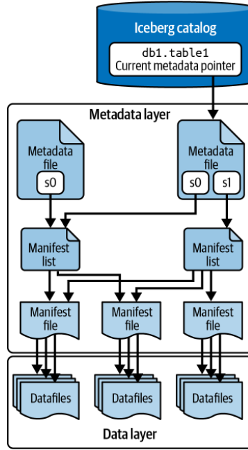
Figure 2.1: Architecture of an Iceberg table, as presented in [22].
