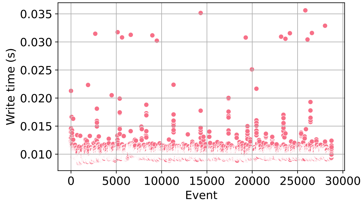
ducklake (duckdb)
