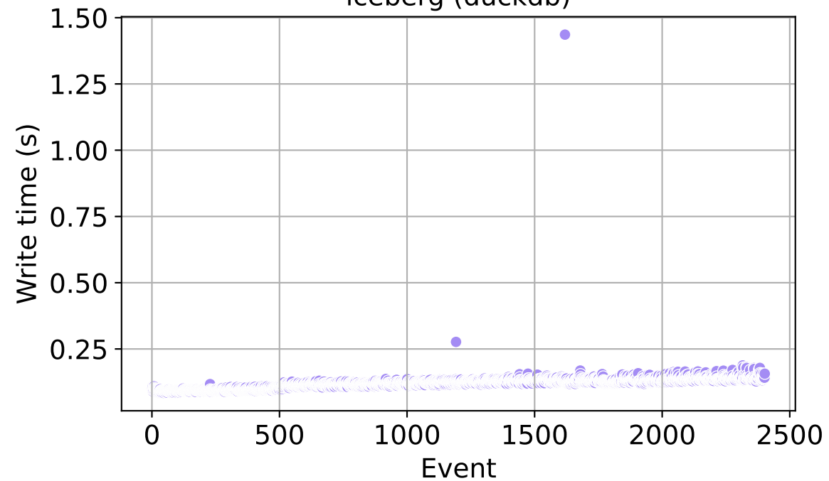
iceberg (duckdb)
