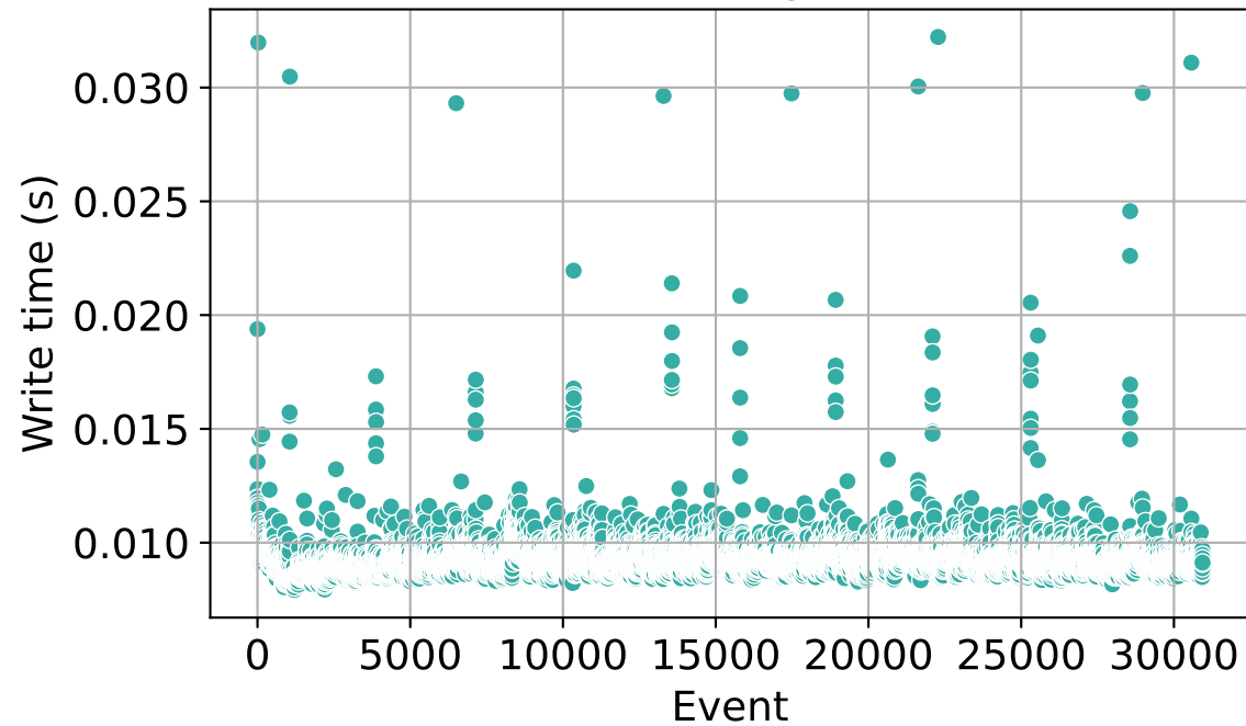
ducklake-inlining (duckdb)
