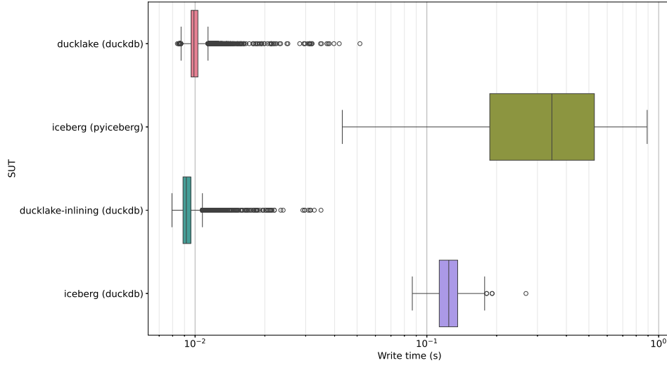
Figure 5.3: Box plots of the time spent writing each individual event to the lakehouse tables during the first warm run, in seconds.
