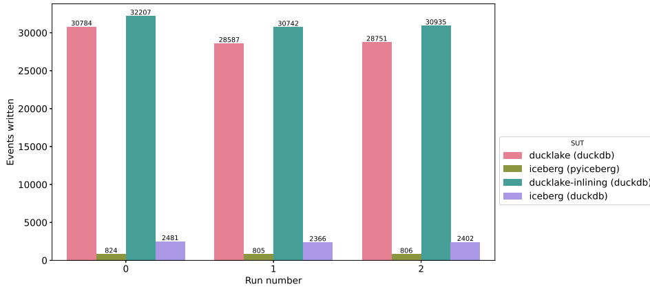
Figure 5.1: Number of events written one by one to each SUT in a time span of 5 minutes. The run numbers correspond to the repetitions of each experiment, where run 0 is considered cold and runs 1 and 2 are considered warm.
