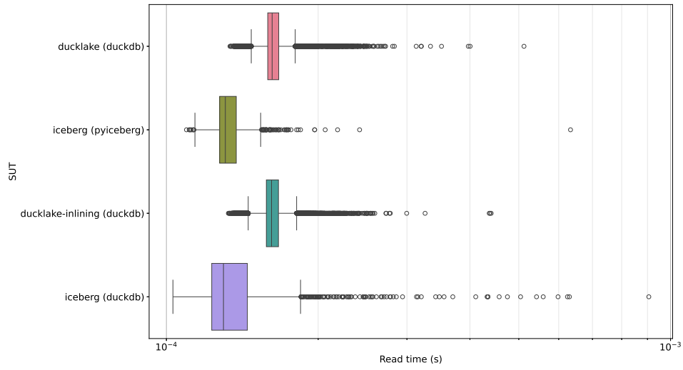
Figure 5.5: Box plots of the time spent reading individual events from Kafka during the first warm run of each SUT, in seconds.
