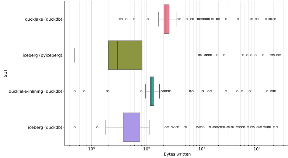
Figure 5.2: Boxplot of bytes written to disk at every second when inserting individual events to each SUT (warm run). The measurements were taken at intervals of 1 second.
