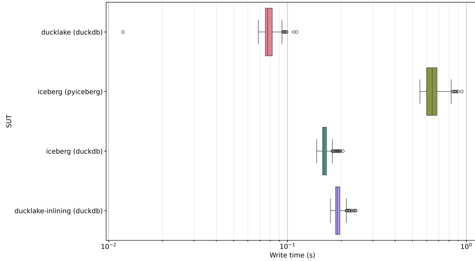
Figure 5.9: Box plots of the time spent writing each batch of 1,000 events to the lakehouse tables during the first warm run, in seconds.
