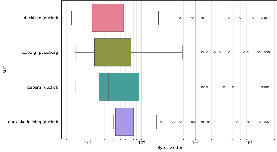
Figure 5.8: Boxplot of bytes written to disk at every second when inserting individual events to each SUT (warm run). The measurements were taken at intervals of 1 second.
