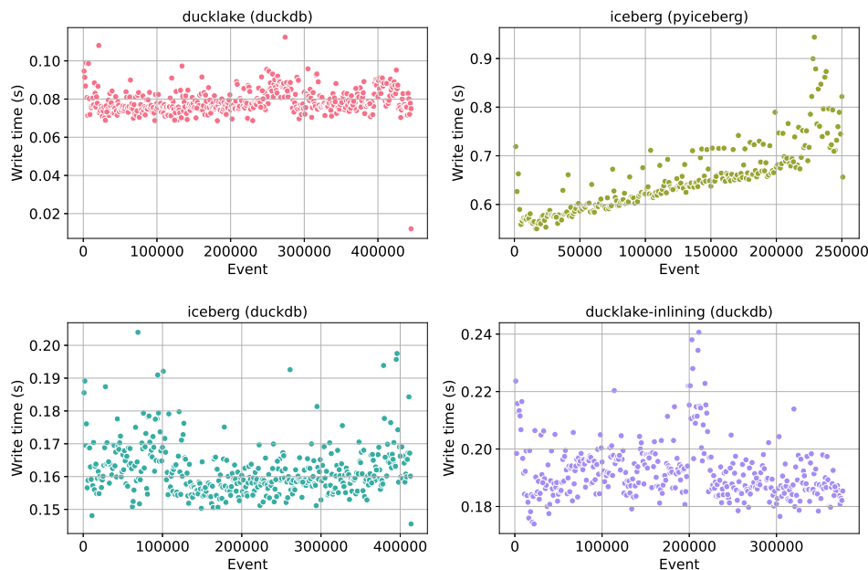
Figure 5.10: Scatter plot of time spent writing batches of 1,000 events to the lakehouse tables during the first warm run, in seconds.
