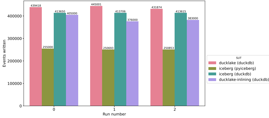
Figure 5.7: Number of events written in batches of 1,000 to each SUT in a time span of 5 minutes. The run numbers correspond to the repetitions of each experiment, where run 0 is considered cold and runs 1 and 2 are considered warm.
