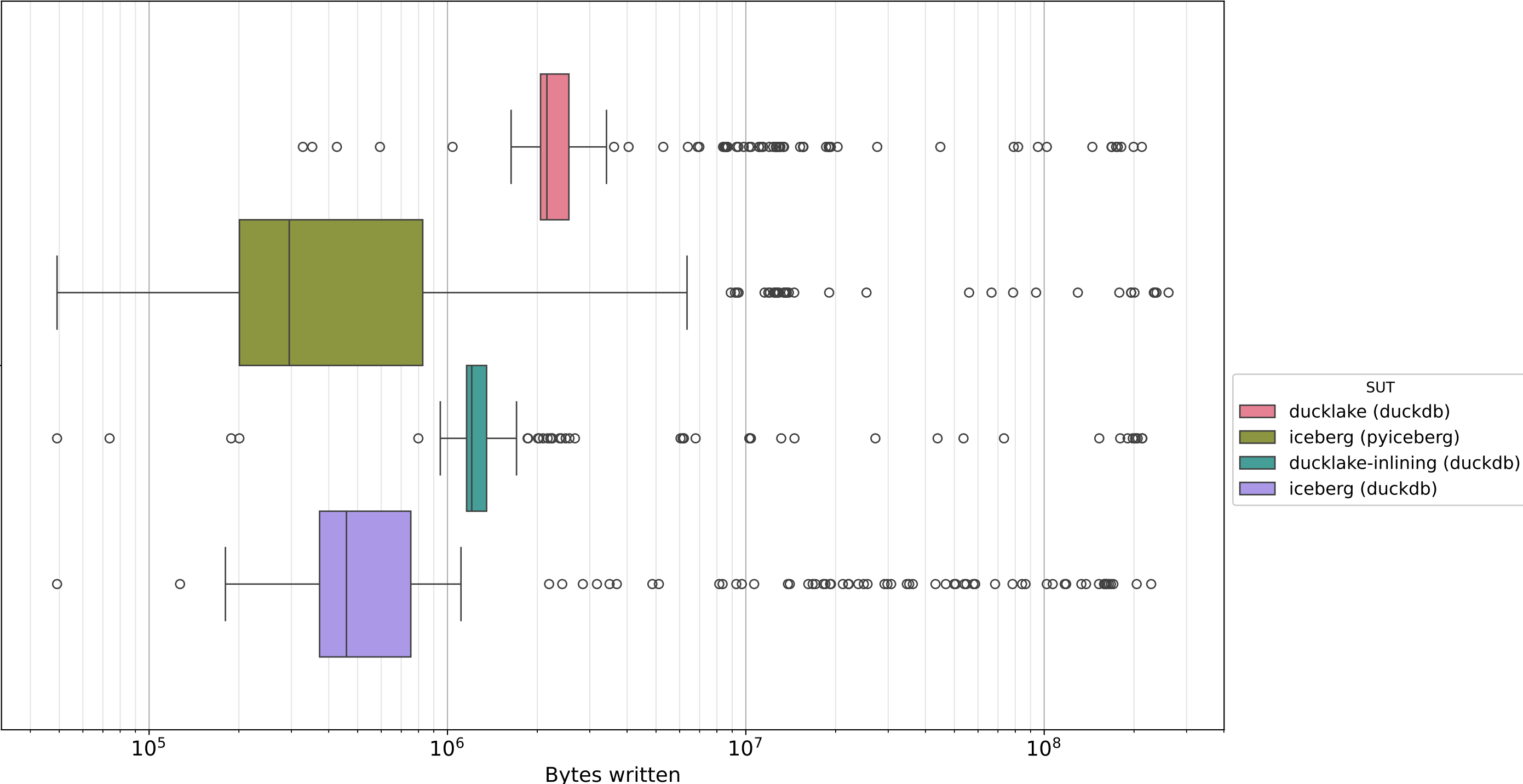
Boxplot of bytes written to disk at every second when inserting individual events to each SUT (warm run)
