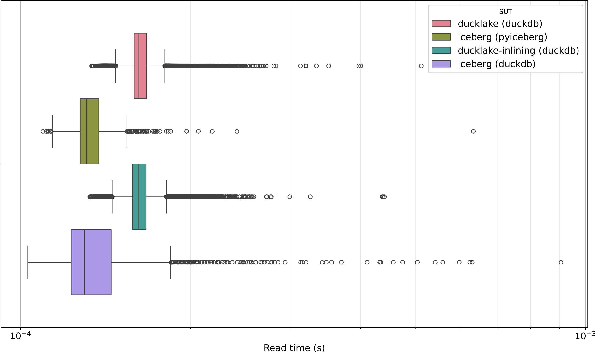
Box plots of the time spent reading individual events from Kafka before inserting them to the SUT, in seconds
