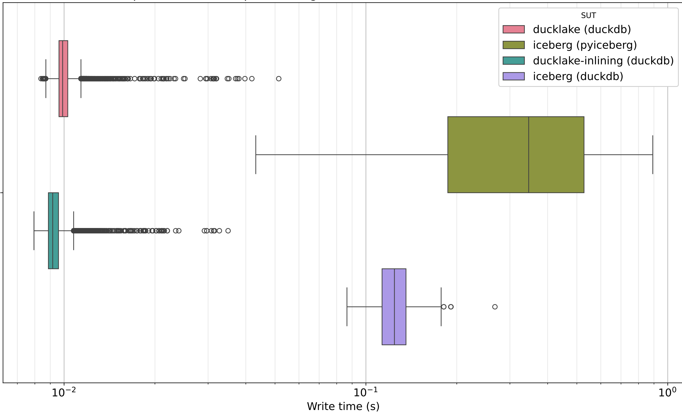
Box plots of the time spent writing individual events for each SUT, in seconds
