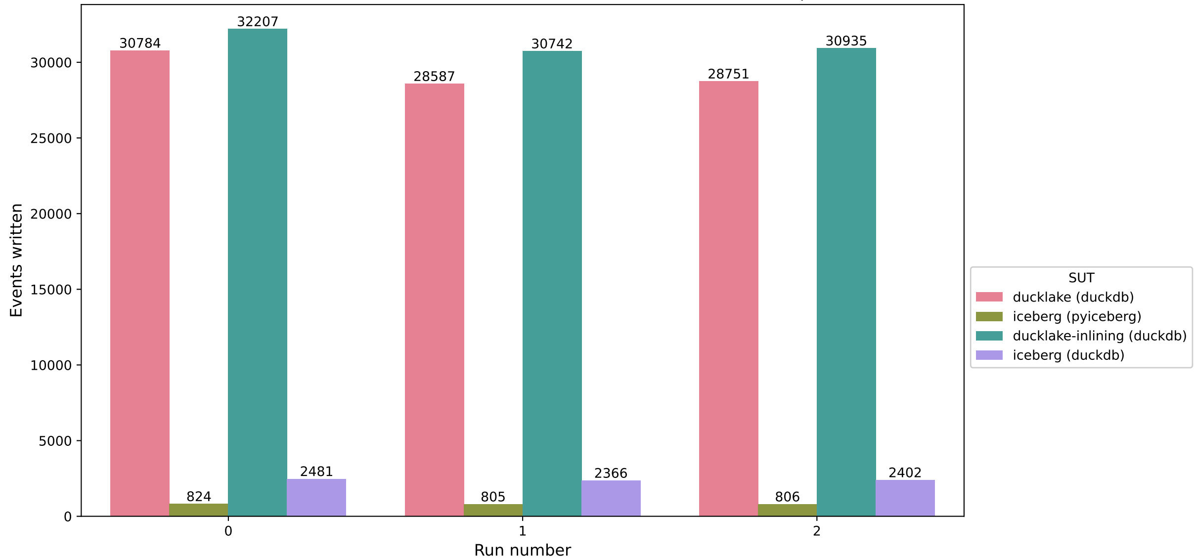
Total number of Kafka events written to each lakehouse after 5 minutes, repeated 3 times
