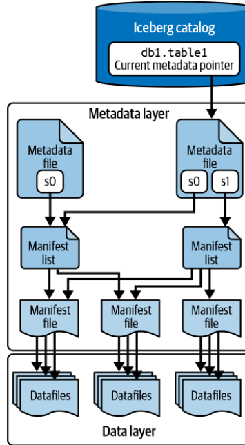
Figure 2.1: Architecture of an Iceberg table, as presented in [21].
