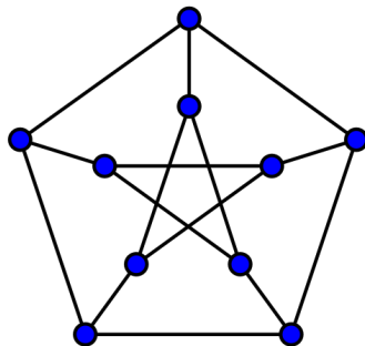
Example of a (3, 5) -graph (Petersen)
