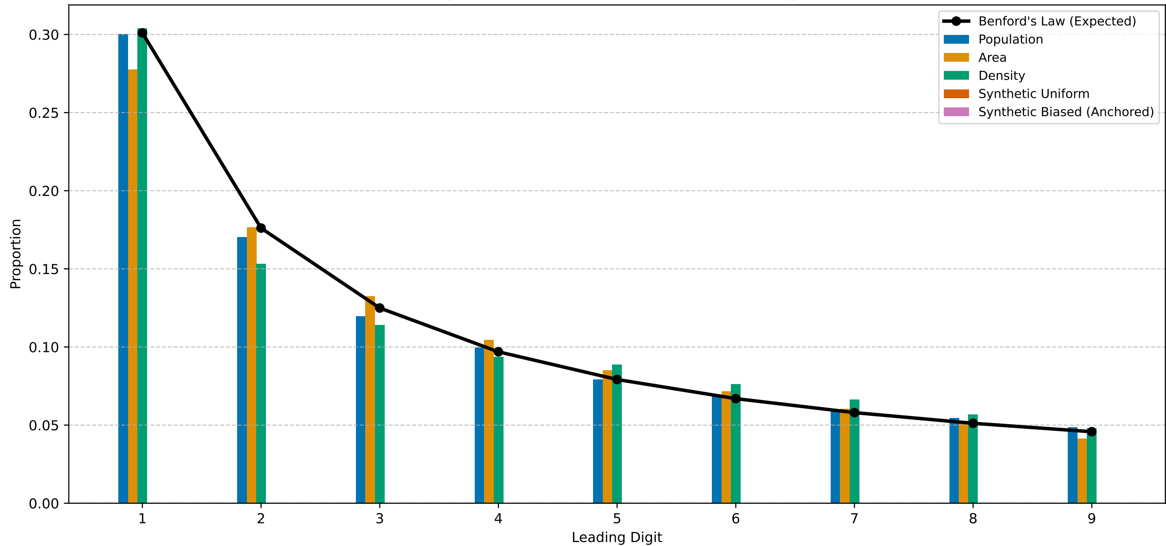
First-Digit Distribution: Observed vs Benford's Expected
