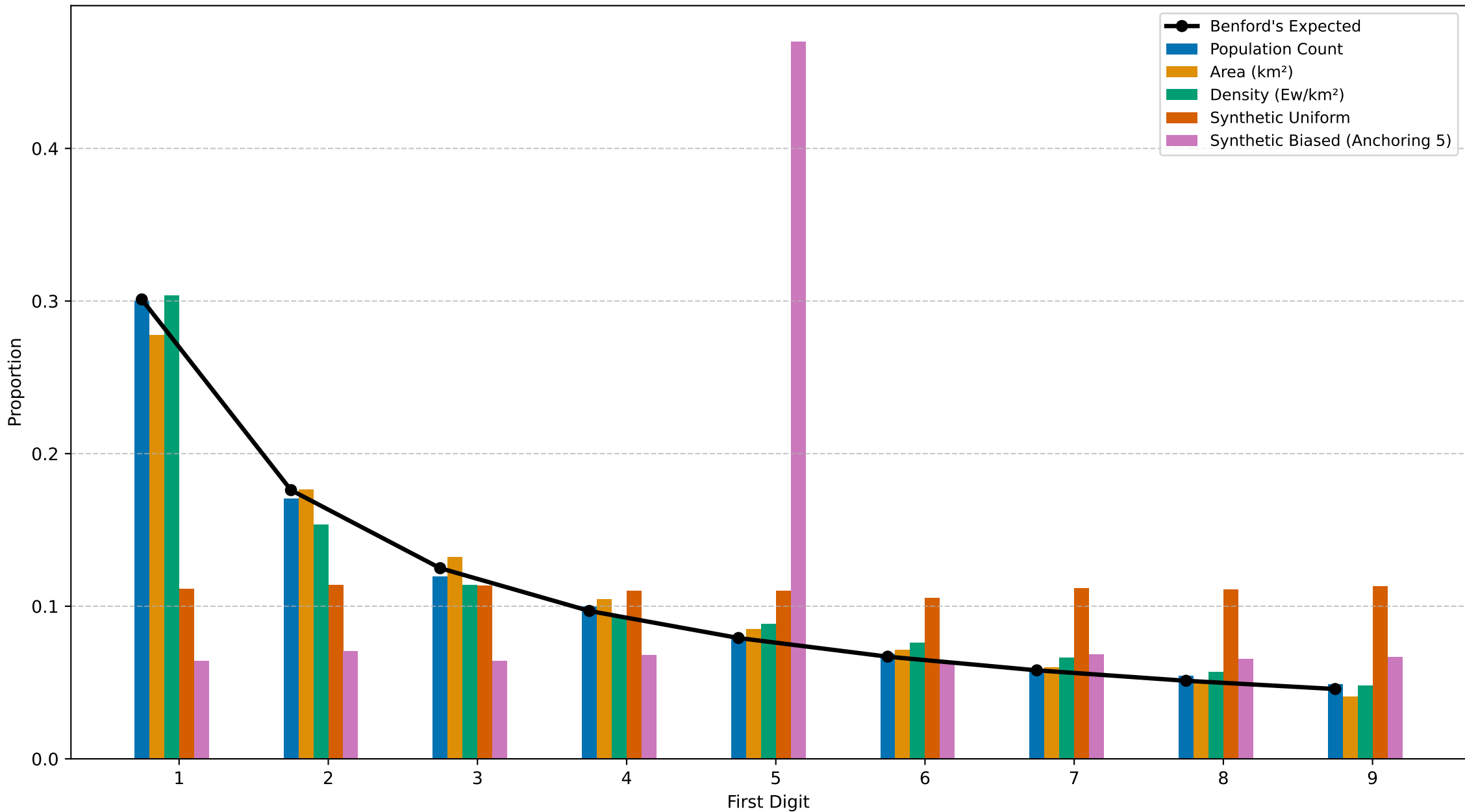
Observed vs. Expected First-Digit Distribution (German Zensus 2022)
