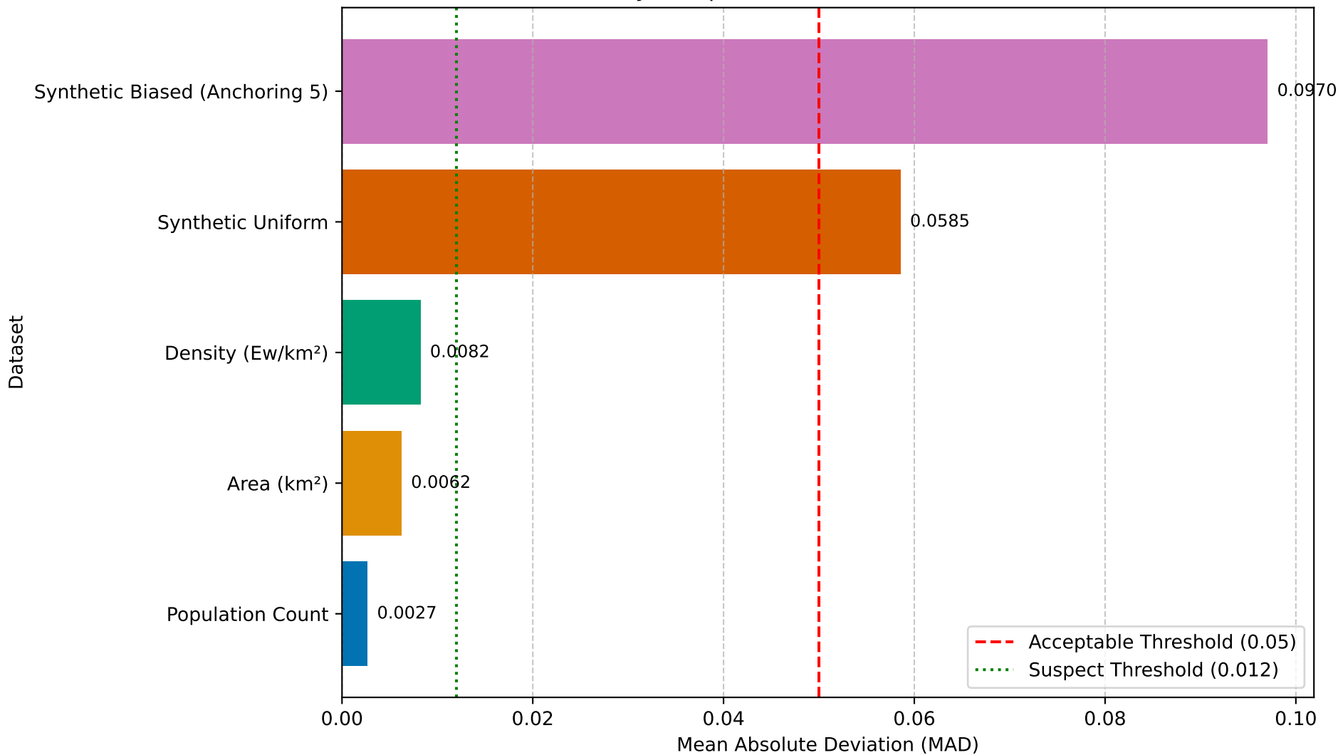
Conformity Comparison: MAD Scores Across Datasets
