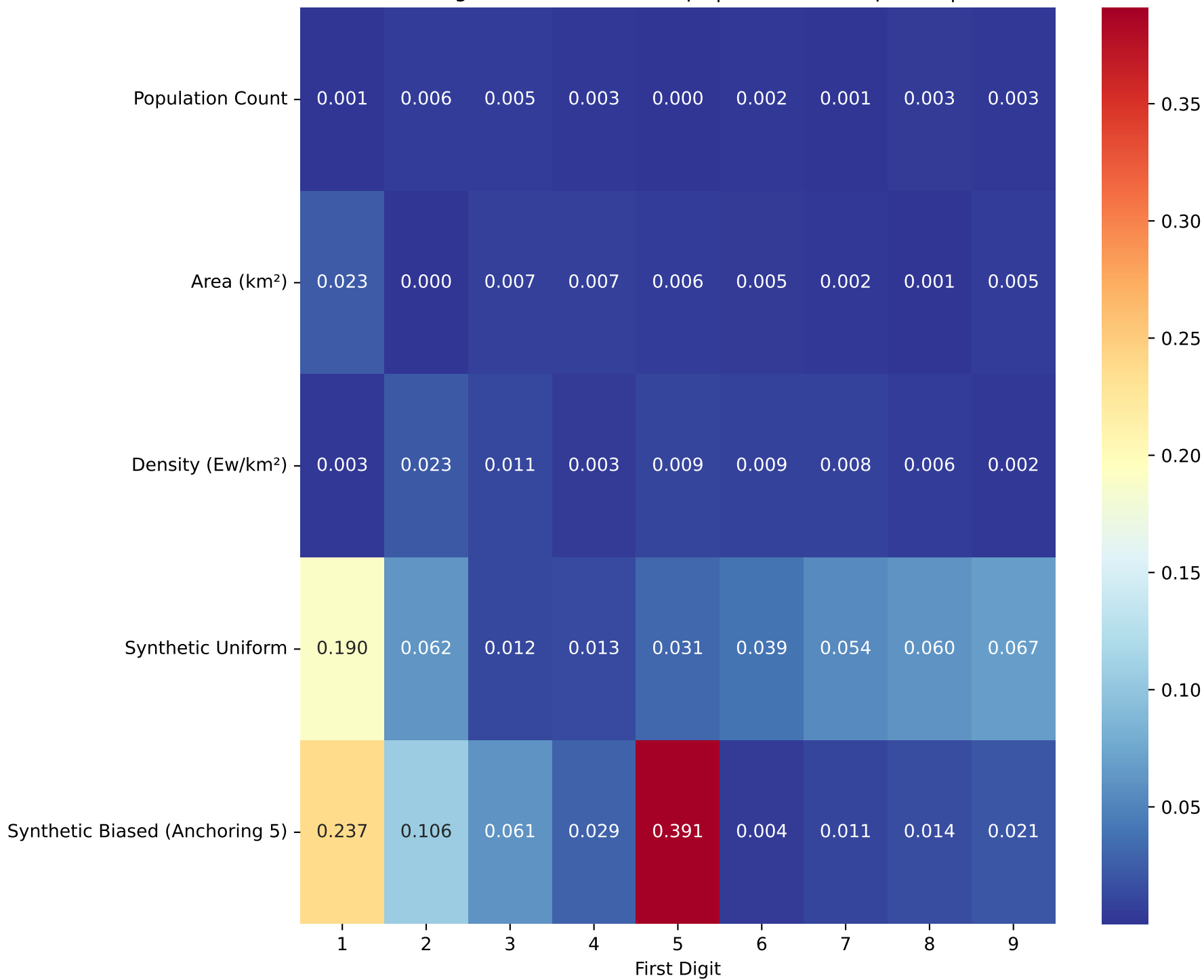
Per-Digit Deviation Heatmap ( |\text{Observed} - \text{Expected}| )
