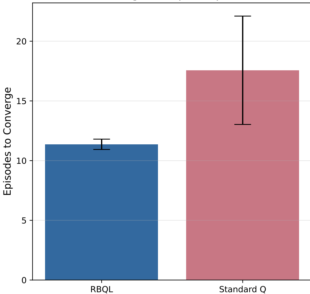
Mean Convergence Speed ( p=9.33e-03 )
