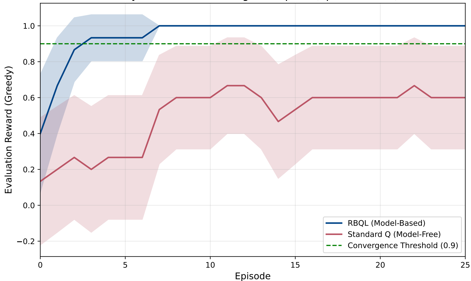
Policy Evaluation: Convergence Speed (Episodes 0-25)
