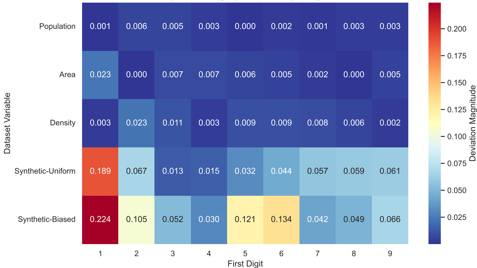
Per-Digit Deviation from Benford's Law (Color intensity = |Observed - Expected|)
