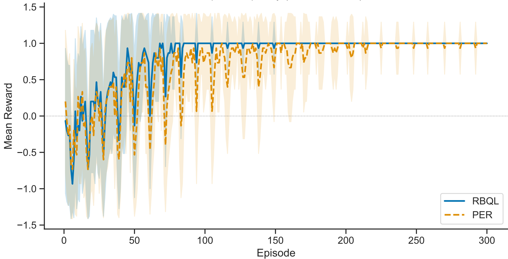
Sample Complexity (30 runs, \pm 1 std)
