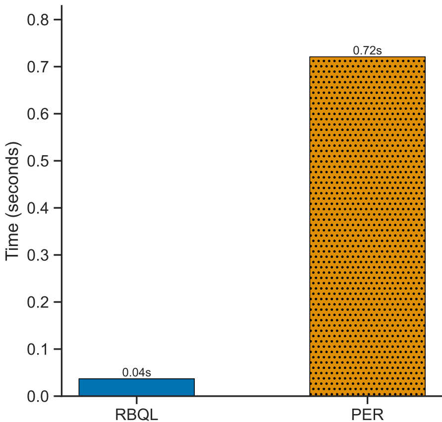
Mean Wall-Clock Time
