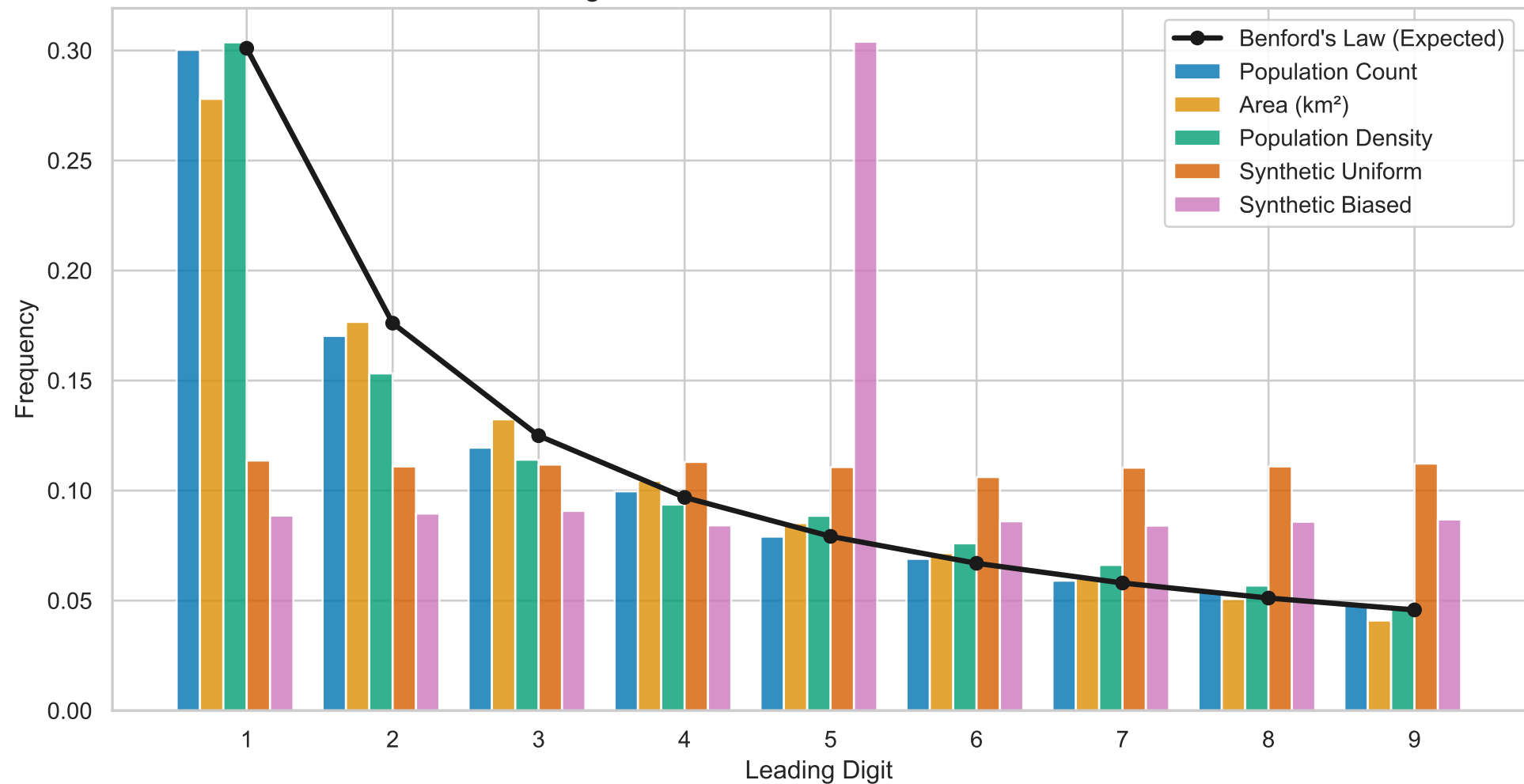
First-Digit Distribution: Observed vs Benford's Law
