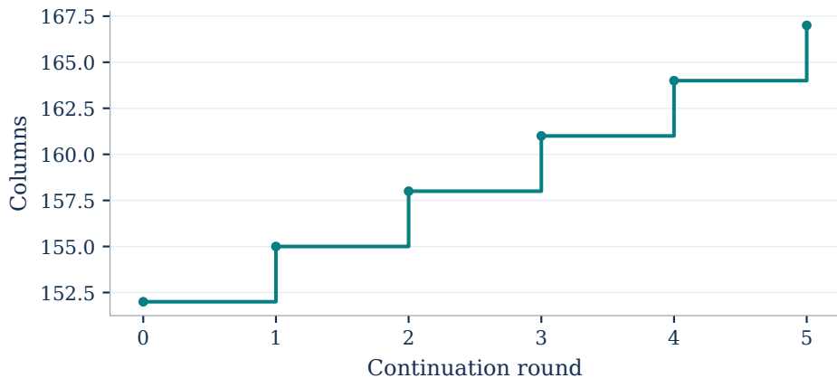
a Restricted-master pool
