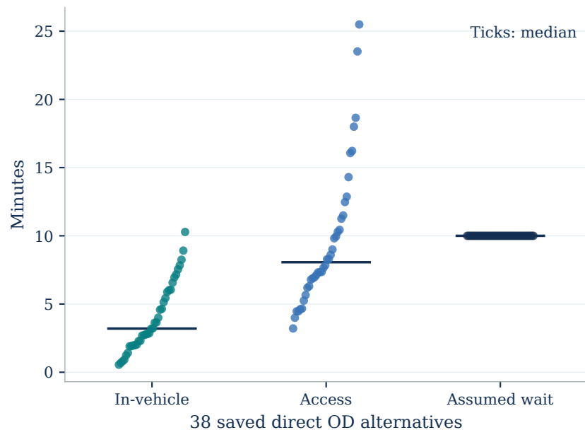
b Saved direct-option components
