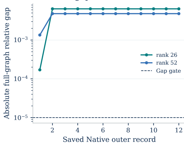
b Native gap
