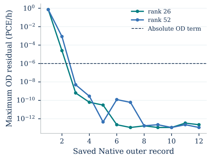
c Native conservation
