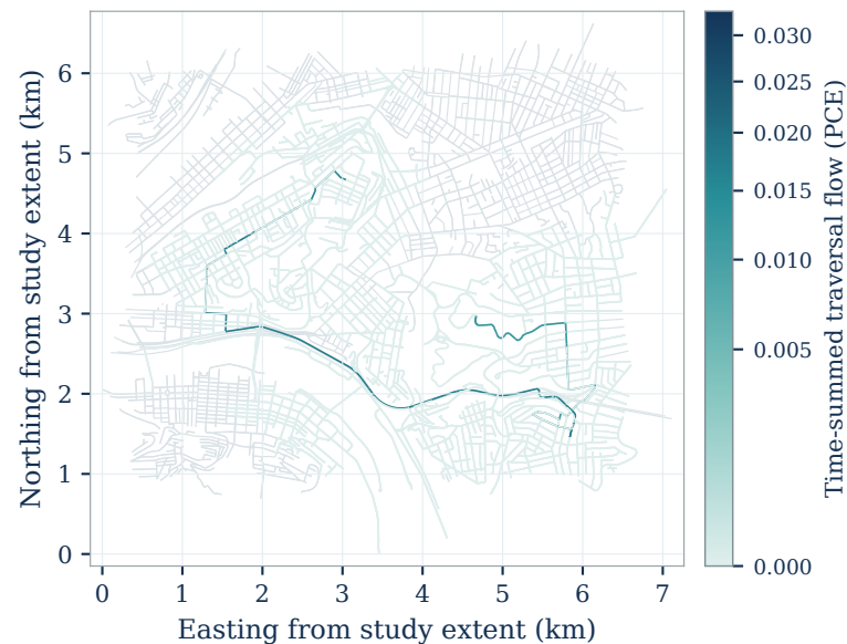
a ADMM · all instantiated physical links
