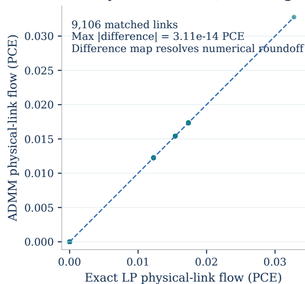
d Every matched link, including zeros
