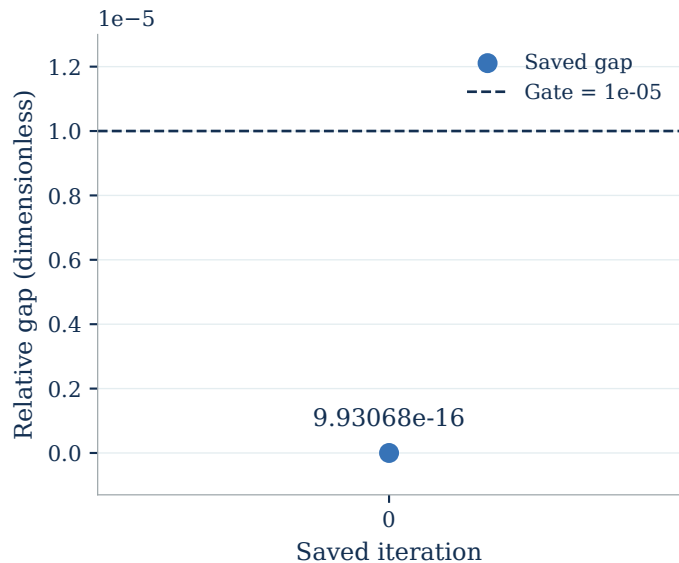
b Relative-gap stopping check
