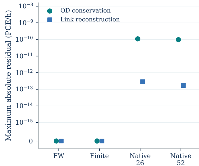
c Original-coordinate feasibility
