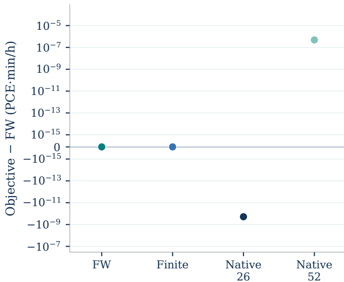
a Objective difference from FW
