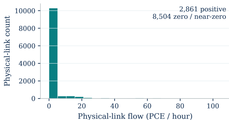
b All-link distribution
