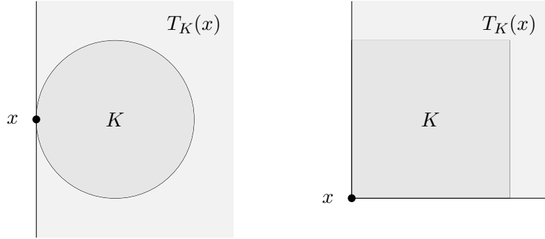
Figure 3.2: Two examples of tangent cones
