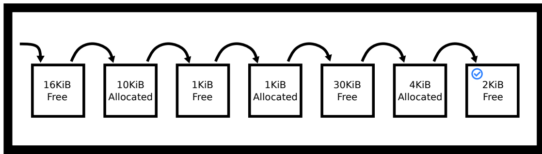
Figure 5.2: Best fit finds an exact match
