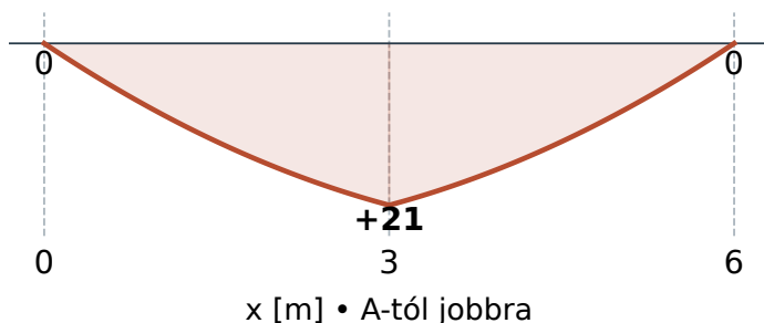
M [kN·m]
