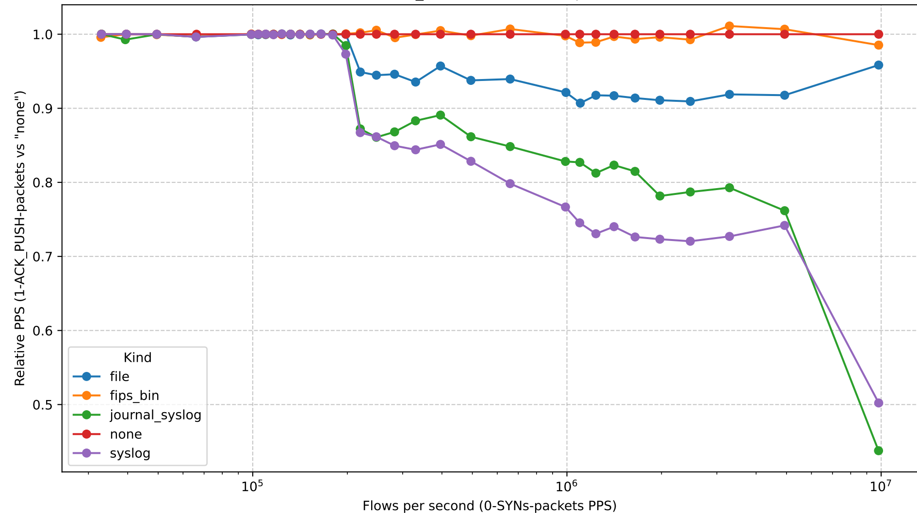
Relative ACK_PUSH PPS vs Flows per Second
