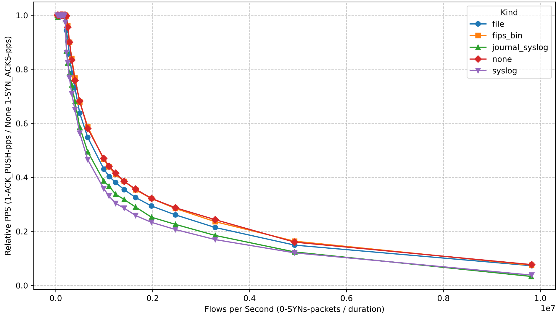
Relative Packets Per Second vs. Flows Per Second
